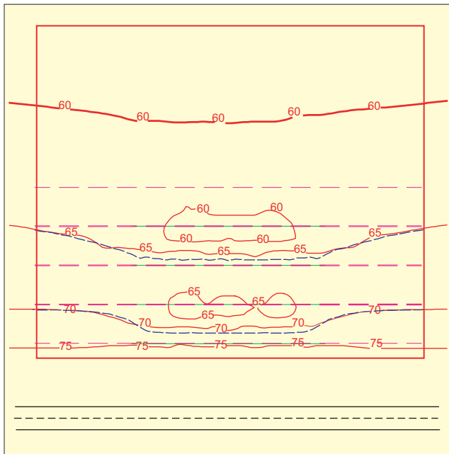
Figure 12. Effect of undulating terrain ( \pm 5 -ft undulations). Contour lines for contour zone: red (with large numbers) = terrain lines within zone, blue (with smaller numbers) = terrain lines outside of zones; green = terrain lines, dashed magenta = contour zones excluding terrain lines.
