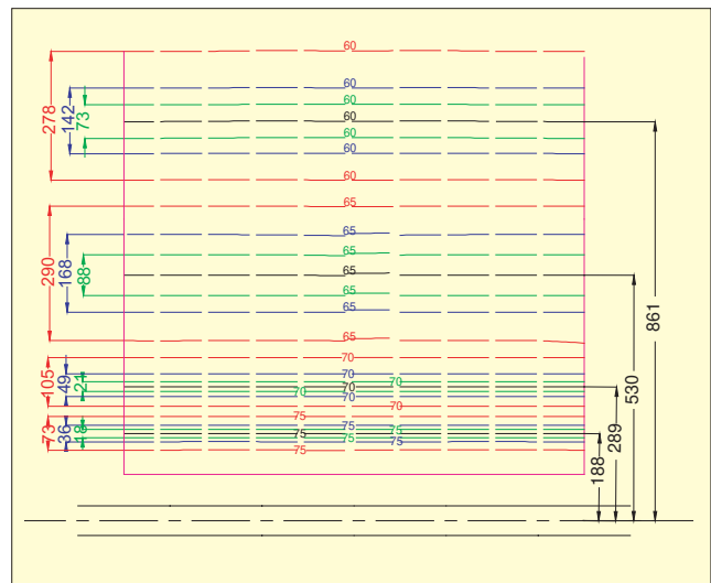
Figure 14. Effect of sound level prediction uncertainty. 75, 70, 65 and 60 dBA contour lines for uncertainty: Black = baseline, green = \pm 0.5 dB, blue = \pm 1.0 dB, red = \pm 2.0 dB.
