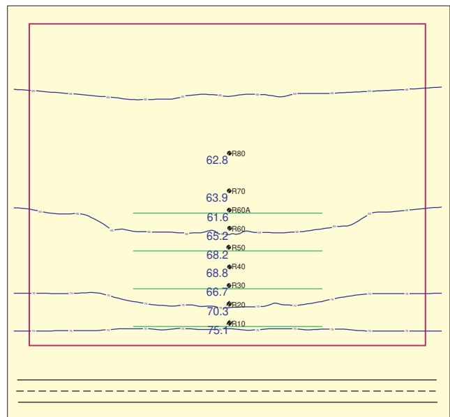
Figure 13. Effect of undulating terrain ( \pm 3 ft undulations). Contour lines for contour zone: blue (with smaller numbers) = terrain lines within zone; green = terrain lines; target symbols = location-specific receptors per Figure 5 with predicted sound levels.
